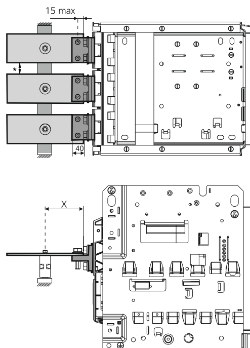
With Terminal Adaptor
