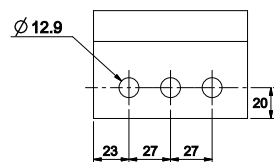
Horizontal Adaptor: CL603160000
