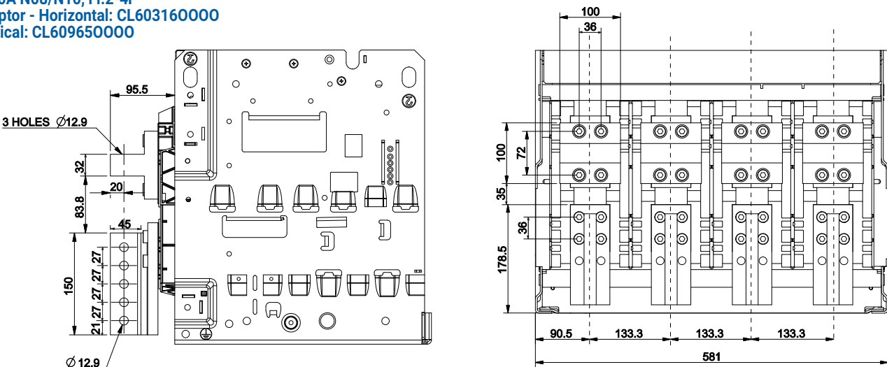
Horizontal Adaptor: CL603160000
