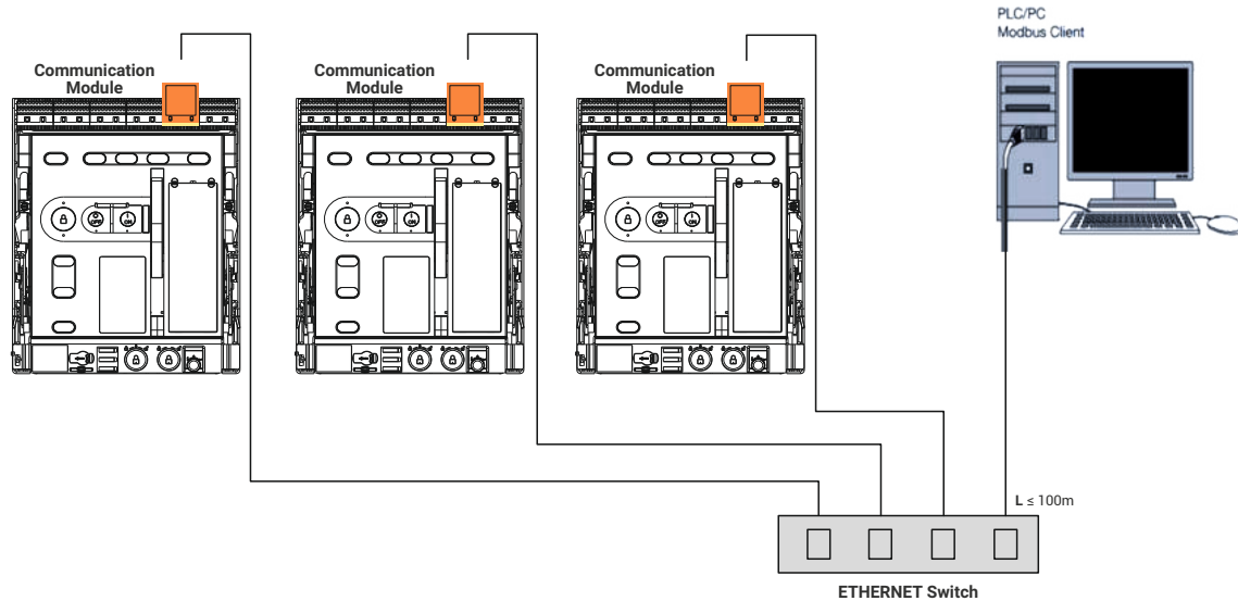
Ref. Diagram : Communication Architecture with OMEGA ACBs
